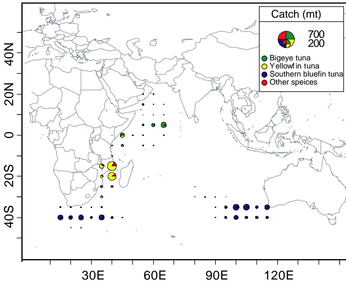
Fig. 2. Catch distribution of tunas and other species in the Indian Ocean by Korean tuna longline fishery in 2008.
