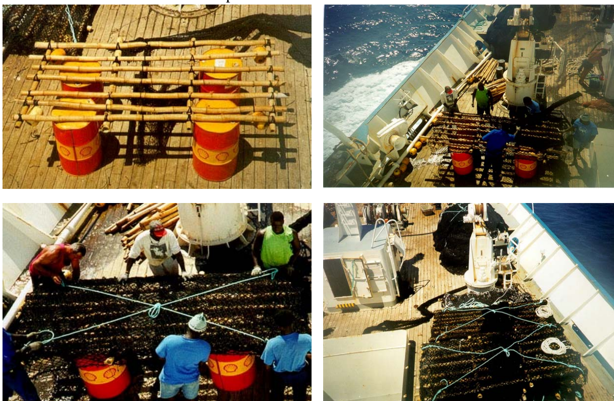
Fig. 4. Building a FAD (© AZTI/isancristobal).
