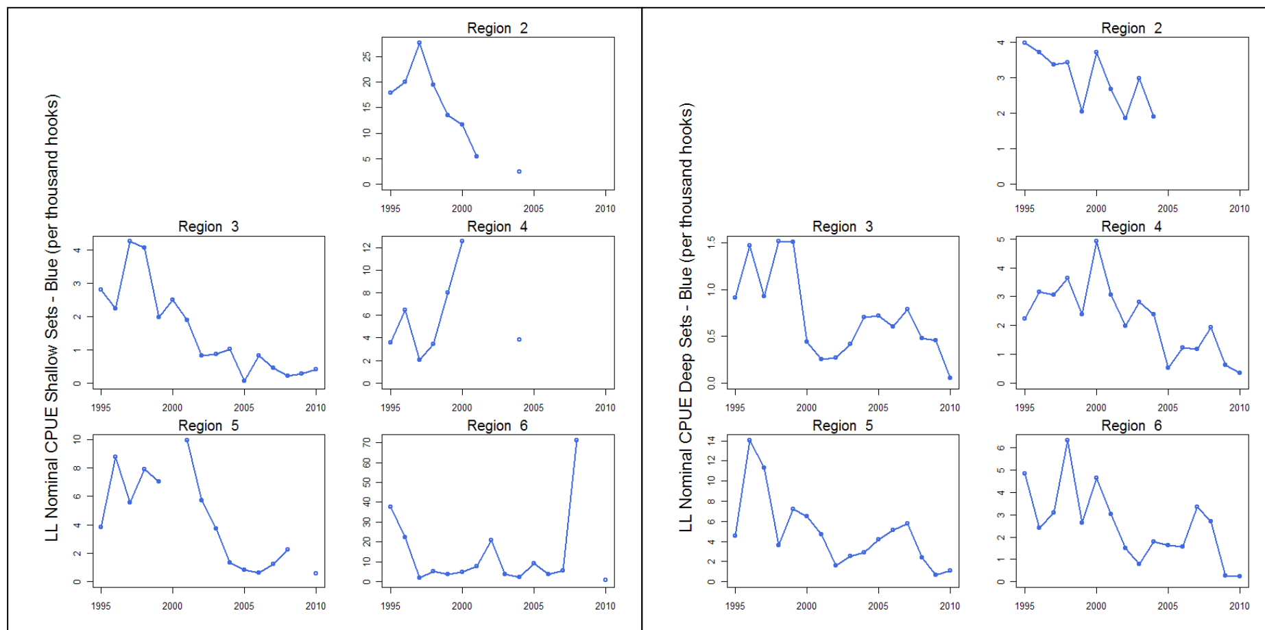
Figure A3. Nominal catch rates by region and year for blue sharks by shallow (<10 hooks per basket) and deep ( \geq 10 hooks per basket) sets.
