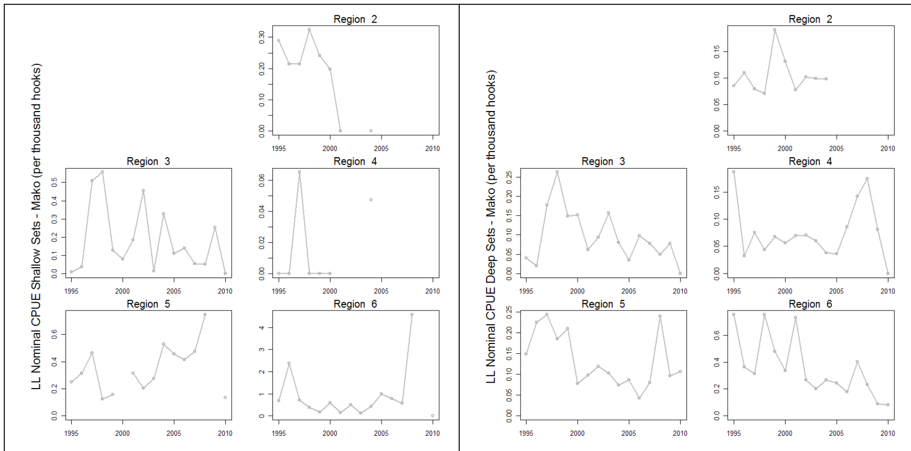
Figure A3 (cont.) Nominal catch rates by region and year for mako sharks by shallow (<10 hooks per basket) and deep ( \geq 10 hooks per basket) sets.
