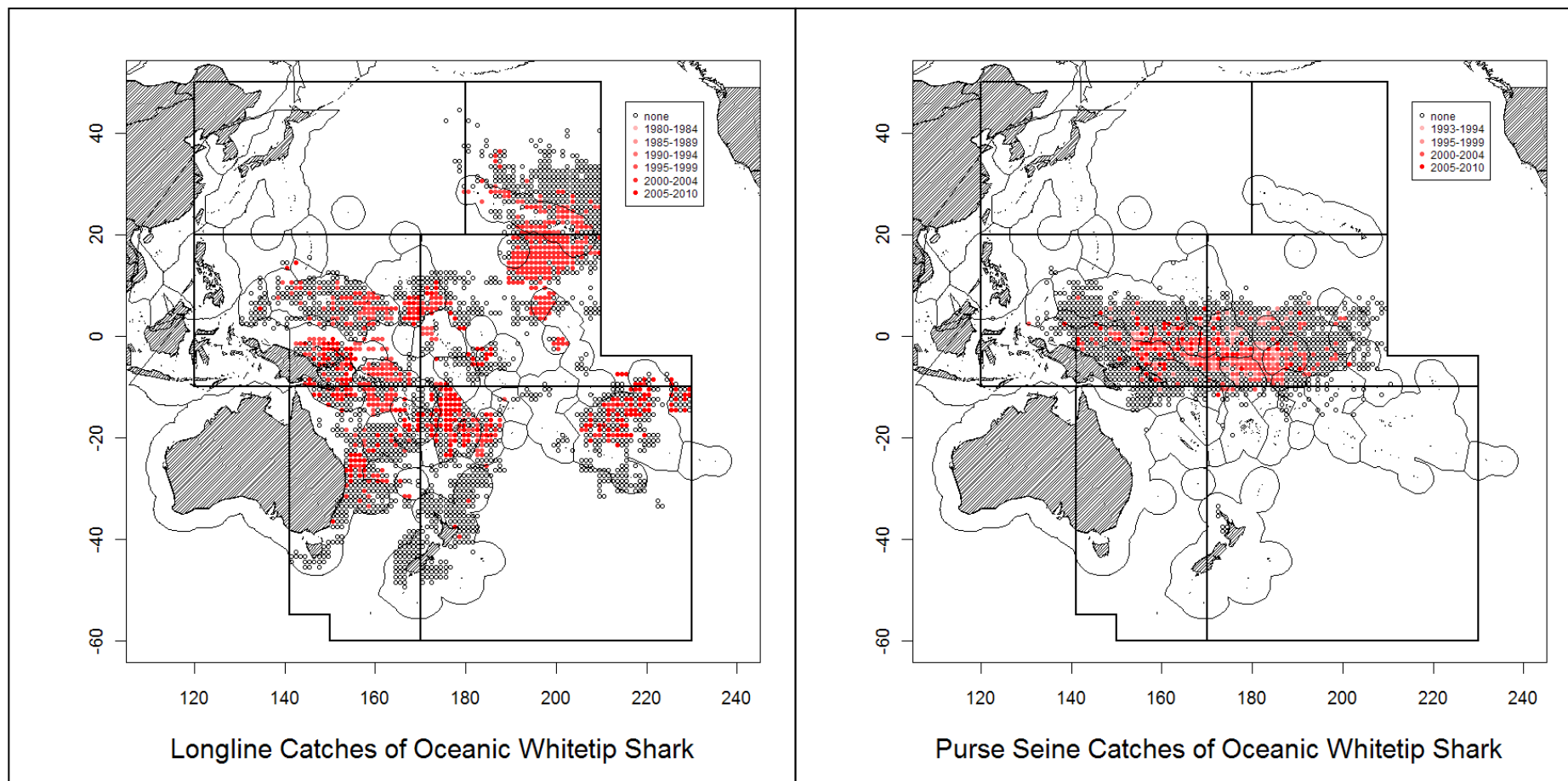
Figure A1 (cont.) Fishery interaction maps for oceanic whitetip (OCS) sharks based on observer records from the WCPO longline (1980-2010) and purse seine fisheries (1993-2010). Colored circles represent positive catches (points are shaded by year with more recent catches in the darkest shades) and empty circles represent zero catch.
