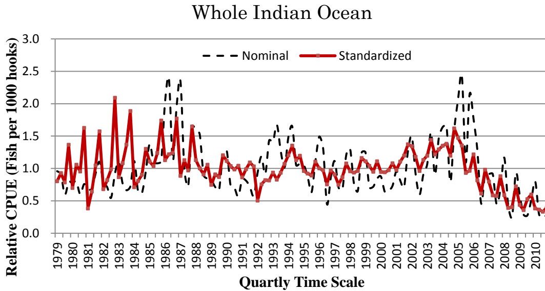
Figure 6. Relative nominal and standardized quarterly CPUE series for the whole Indian Ocean from 1979 to 2010.
