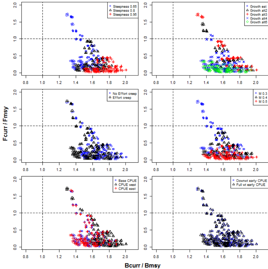
Figure 55: Scatter plots of values estimated under a grid of scenarios for steepness, assumptions about growth, effort creep, natural mortality, CPUE, and early CPUE. Response variables are F_{\text{current}} / F_{\text{MSY}} versus the spawning potential depletion ratio SB_{\text{current}} / SB_{\text{MSY}} .
